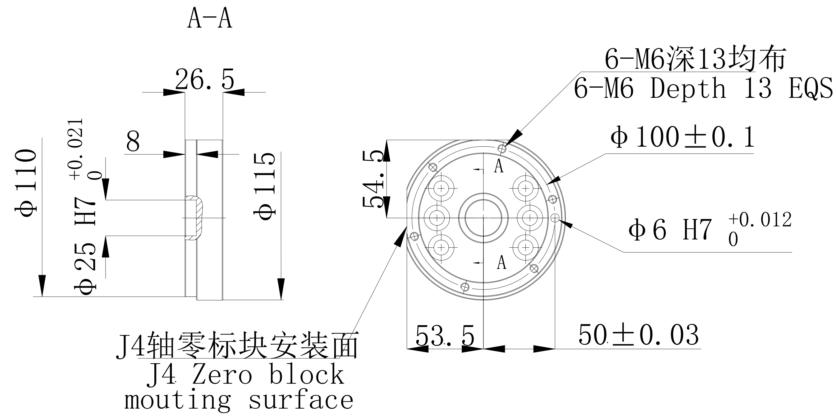
底座安装尺寸 Base mounting size
