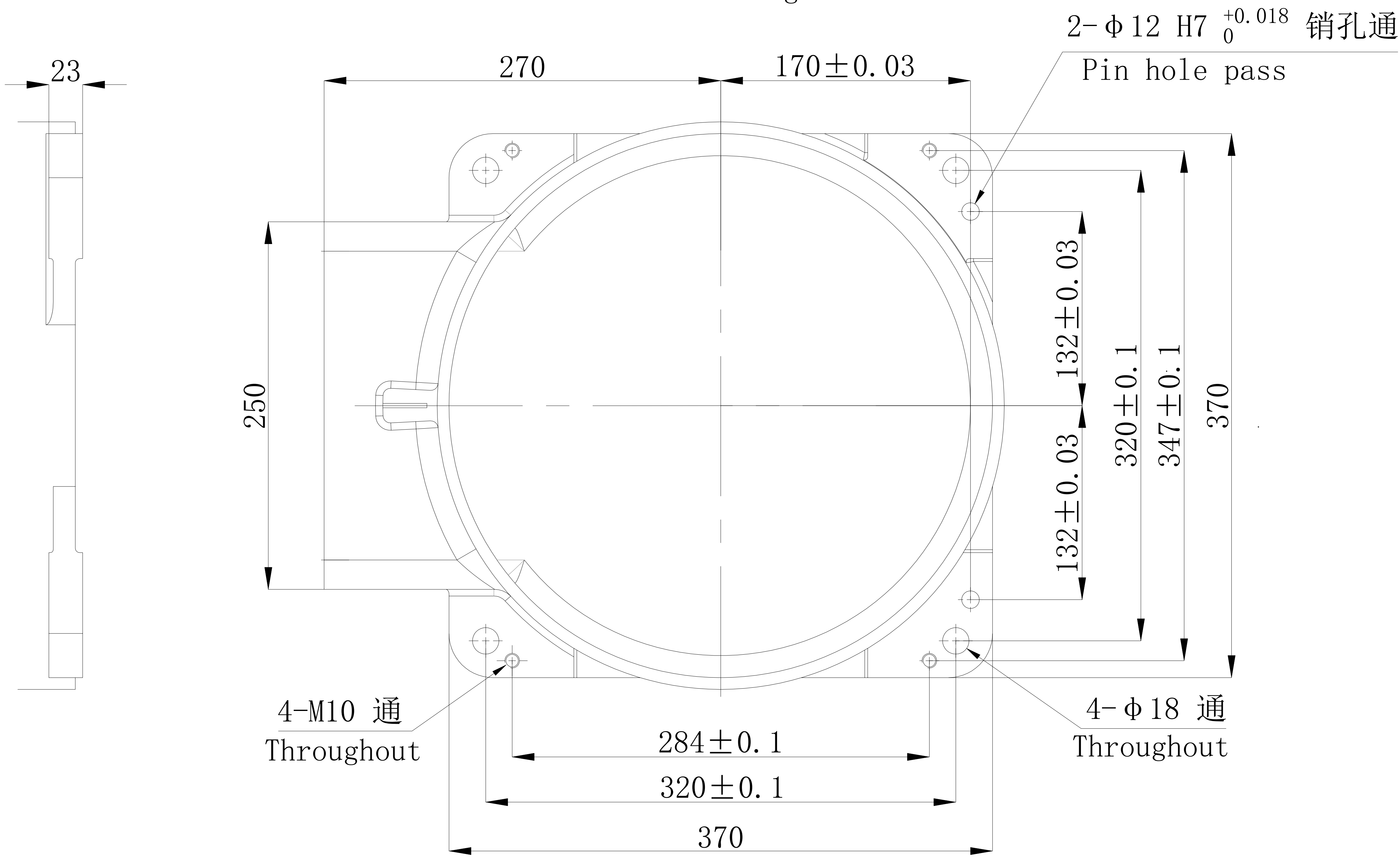
底座安装尺寸 Base mounting size
