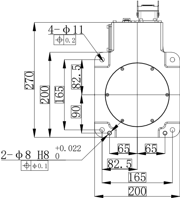
底座安装图(Base mounting size)
