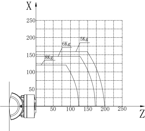
负载曲线图(Load curve)
