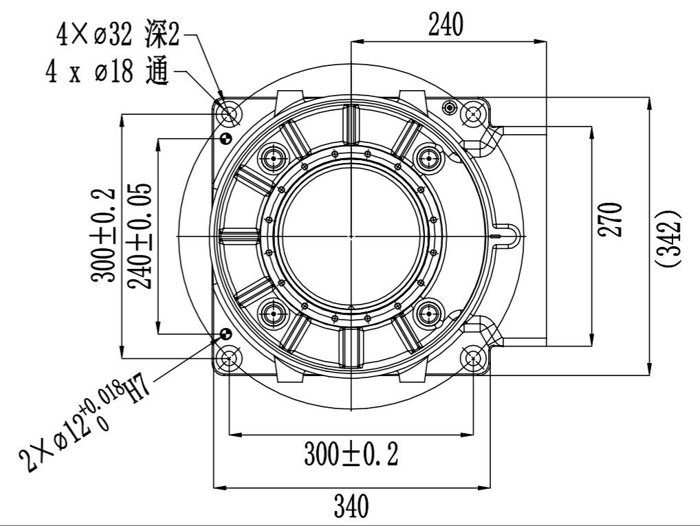
End flange mounting size diagram 末端法兰安装尺寸图
